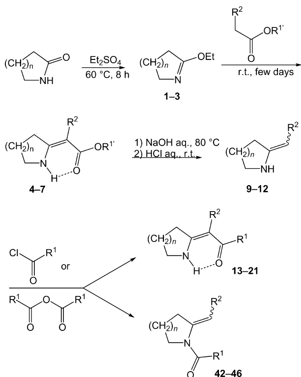
Scheme 1. Synthesis of ligands containing R^3, R^4 = -(CH_2)_n- with n = 3, 4, 5 .
