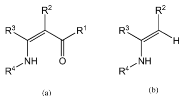
Figure 2. General formula of the ligands (a) and ligand precursors (b) synthesised.
