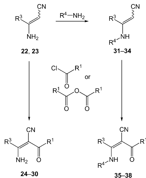
Scheme 2. Synthesis of ligands containing individual substituents R^3 and R^4 ( R^2 = \text{CN} ).
