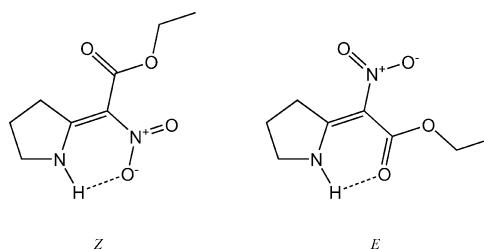
Figure 3. E/Z Isomerism of ligand 7 .
