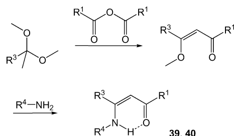
Scheme 3. Synthesis of ligands containing R^2 = H .
