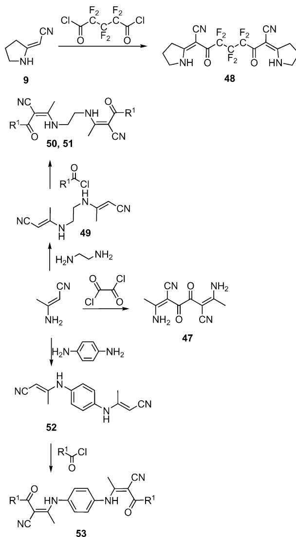
Scheme 4. Synthesis of ligands bearing two N,O-bidentate \beta -enaminonic coordination sites.
